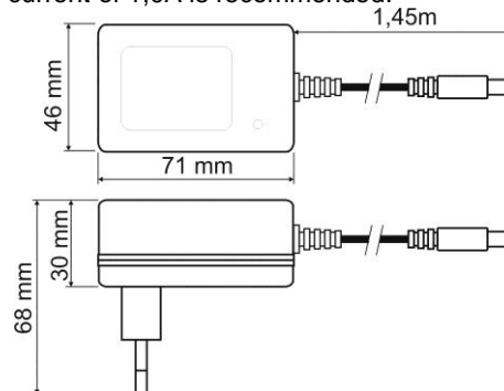
Fig.1. Dimensions of power supply.
