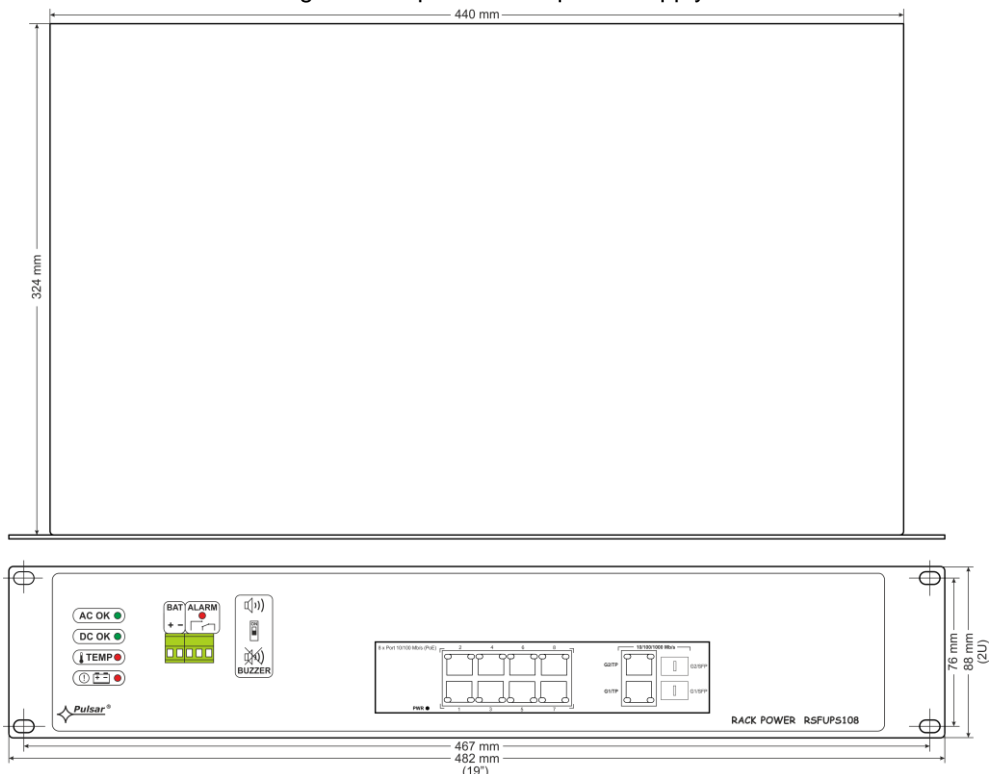
Fig.4. The view of the PSU.
