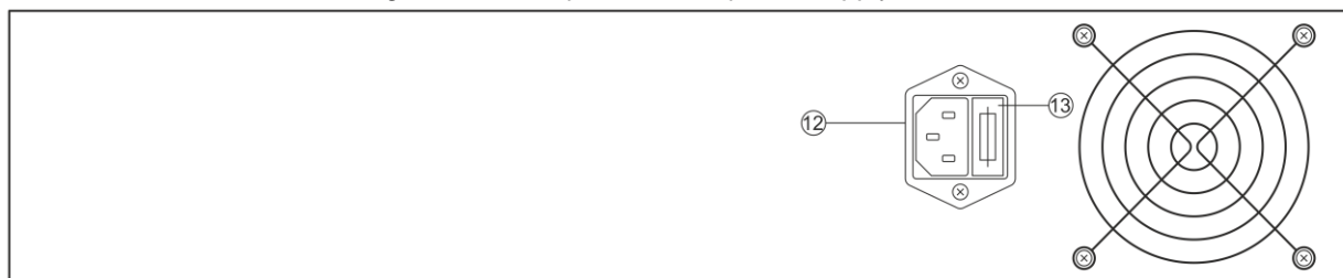
Fig. 3. Rear panel of the power supply.
