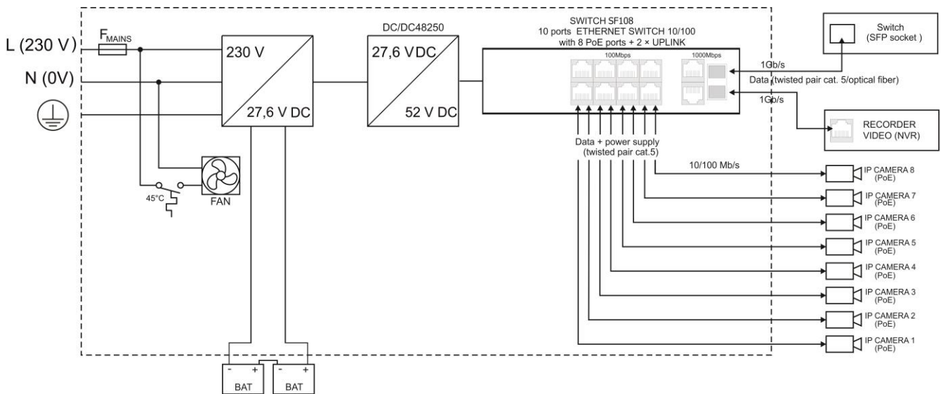
Fig.1. The block diagram of the PSU.
