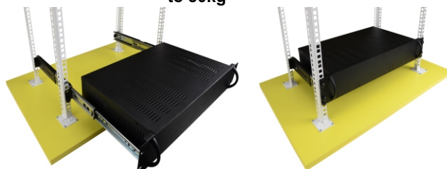
Mounting with the ARAS450 rails to 30kg
